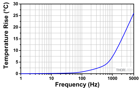
Temperature Rise vs. Drive Voltage Frequency
