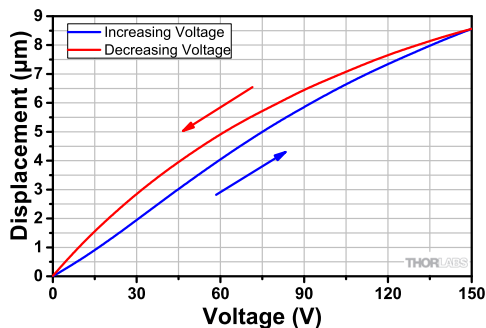
Displacement (No Load, 25 °C, 150 V Max)
