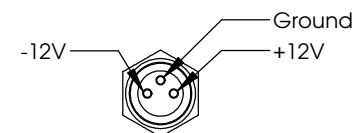
Electrical Connections
