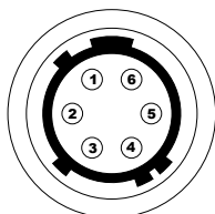
HIROSE CONNECTOR*
