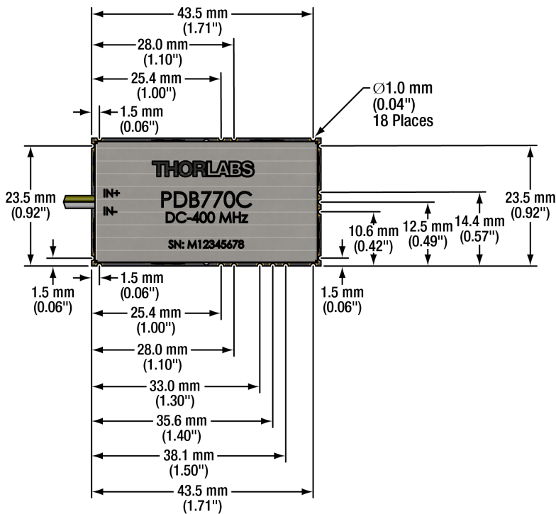
Top View PDB770C
