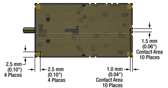
Bottom View PDB770C
