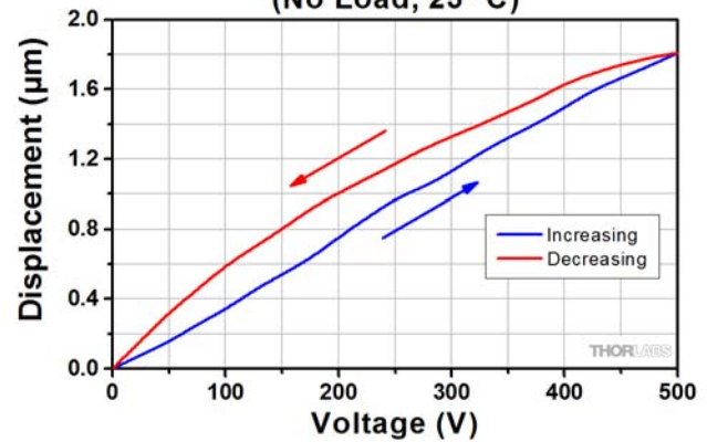
PT49LM(W) Radial Displacement (No Load, 25 °C)
