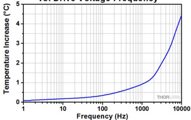
PT49LM(W) Temperature Increase vs. Drive Voltage Frequency
