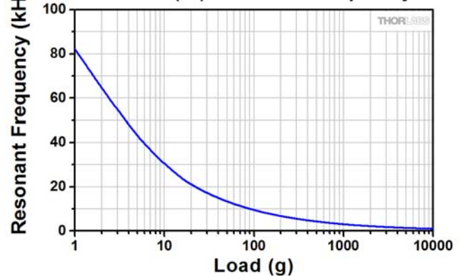
PT49LM(W) Resonant Frequency
