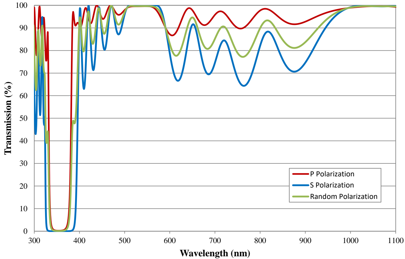
532 & 1064nm T, 355nm R Harmonic Separator Typical Transmission FOR REFERENCE ONLY
