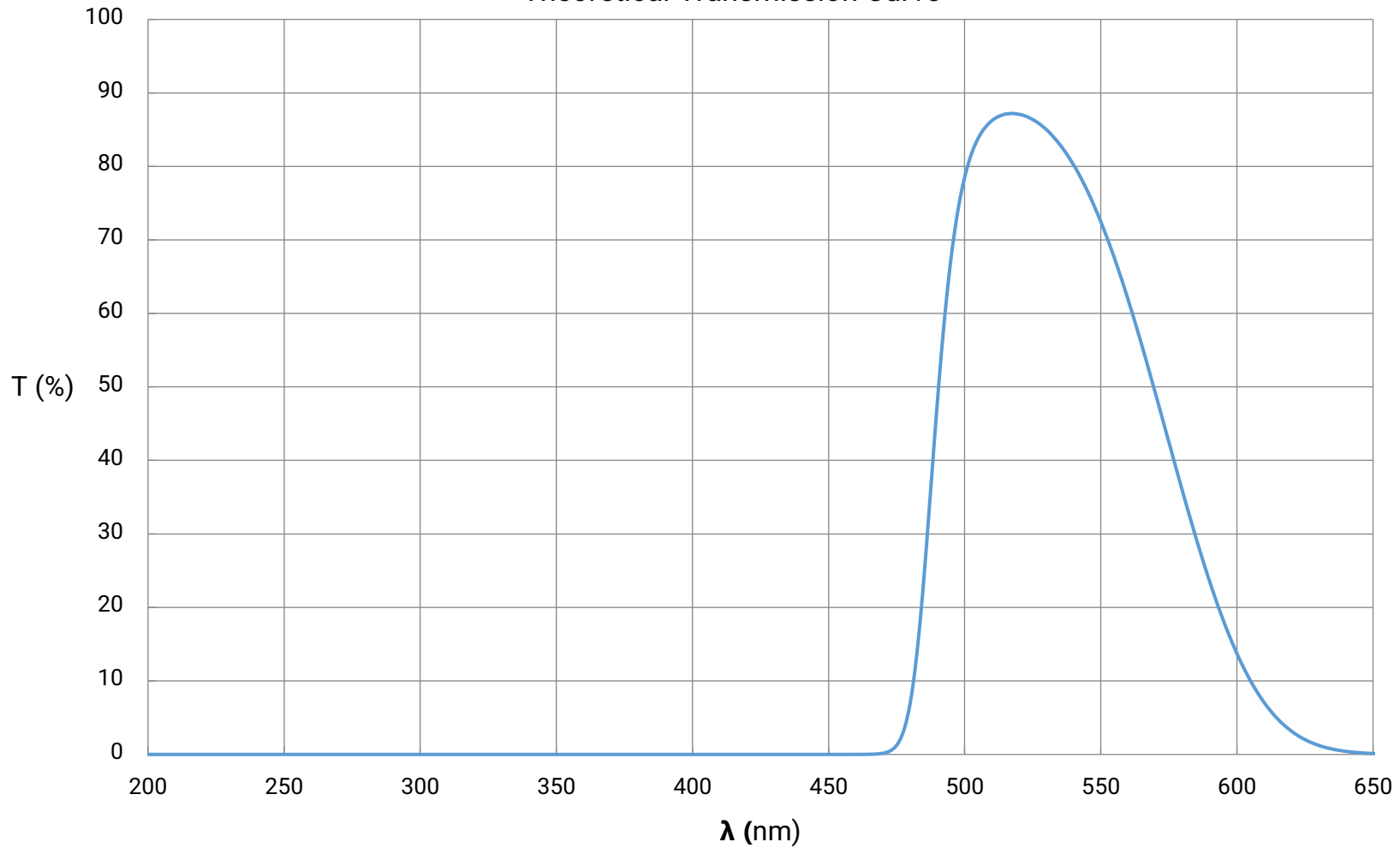
Astronomy Bandpass Filter, Violet Theoretical Transmission Curve
