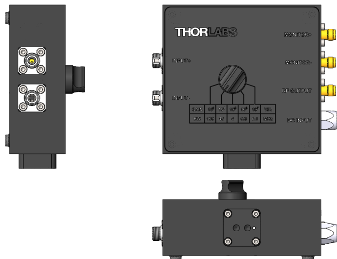
Adapter plate mounting positions Option A
