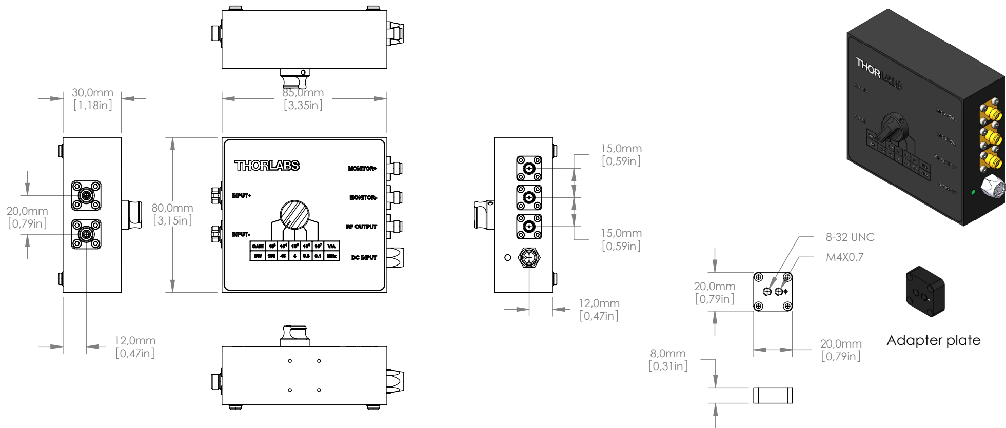
Adapter plate mounting positions Option A
