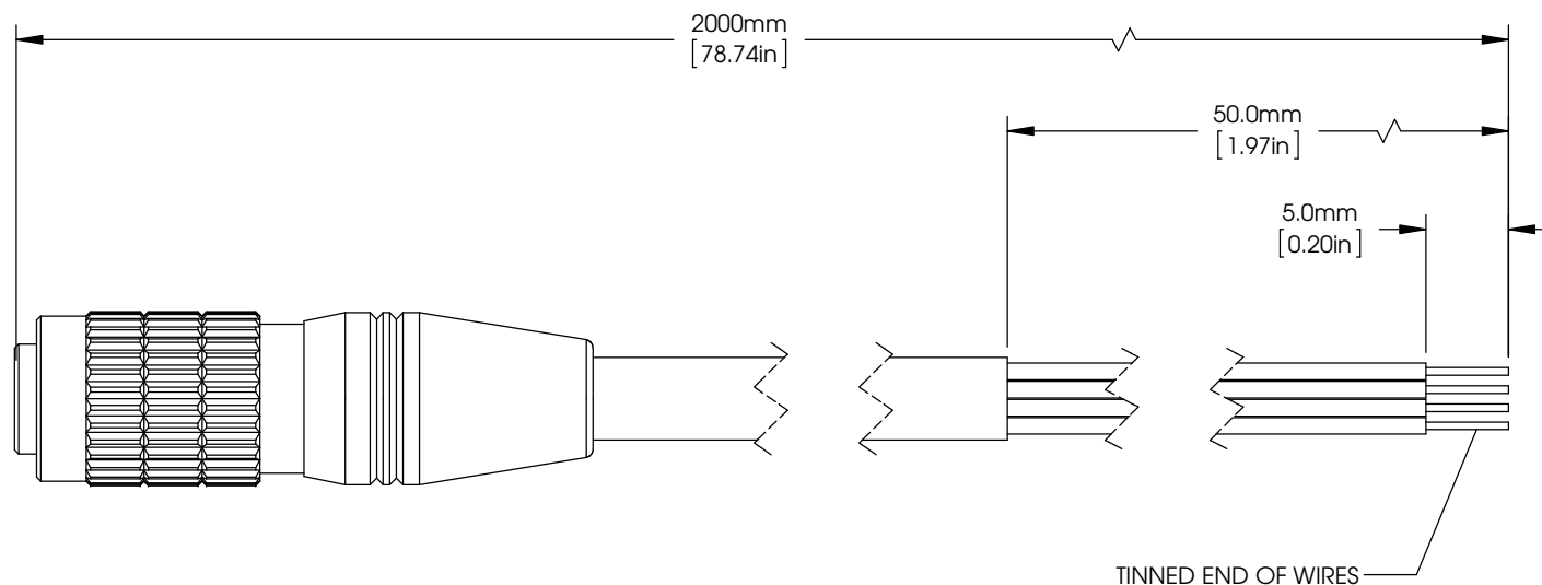
CONNECTOR: HIROSE HR25-7TP-8S(72)
