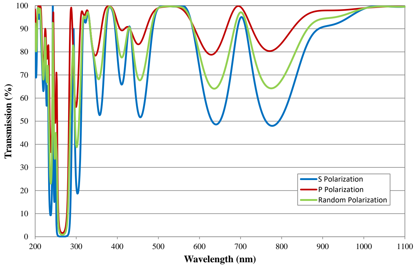
532 & 1064nm T, 266nm R Harmonic Separator Typical Transmission FOR REFERENCE ONLY
