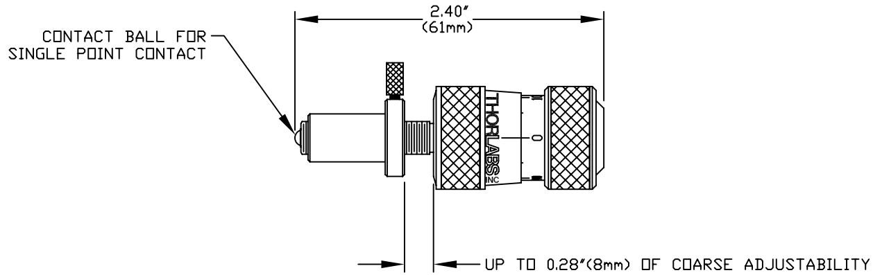
FINE ADJUSTMENT FULLY RETRACTED
