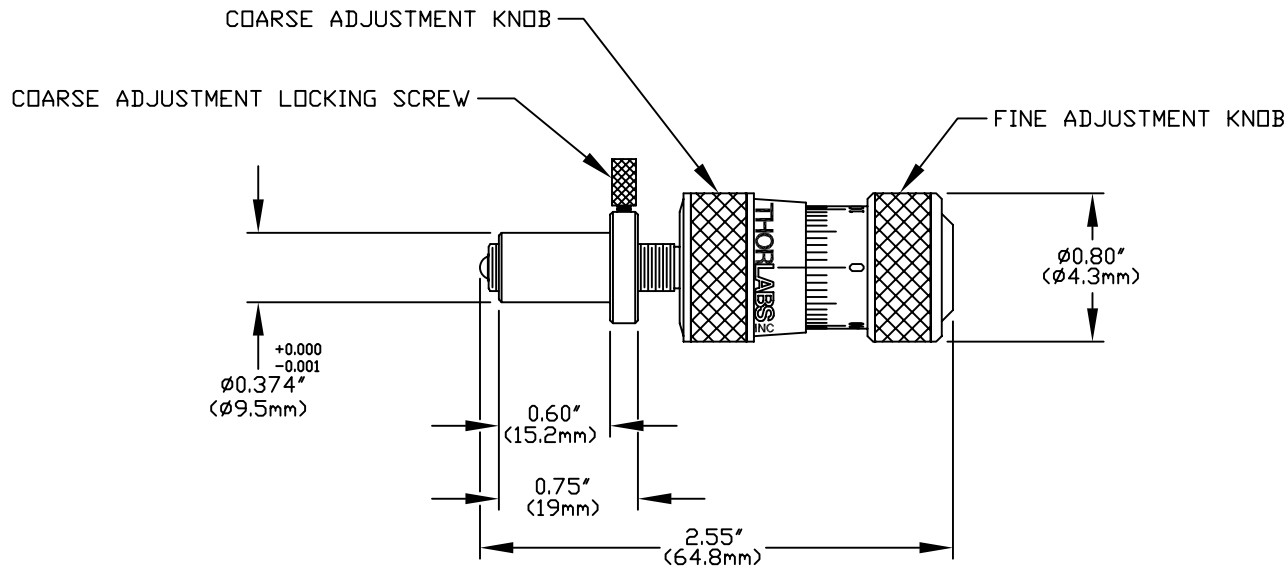
FINE ADJUSTMENT FULLY EXTENDED
