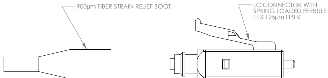
EXPLODED VIEW
