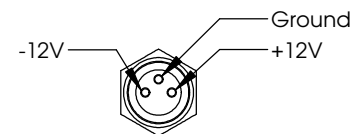
Electrical Connections
