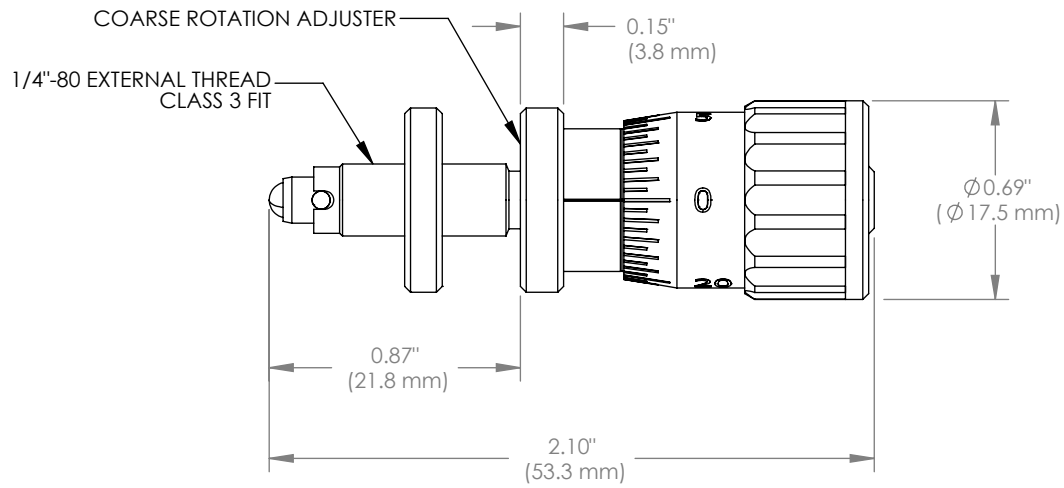
SPINDLE FULLY RETRACTED VIEW
