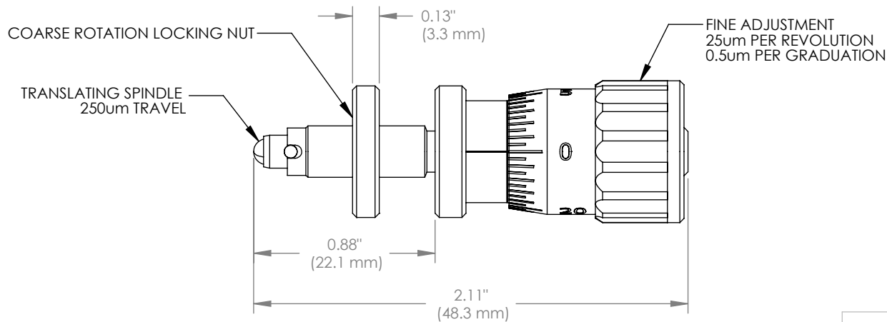
SPINDLE FULLY EXTENDED VIEW
