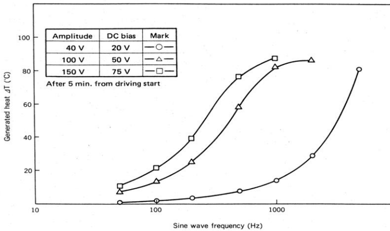
Figure 1- Sine wave Frequency vs. Generated Heat
