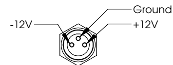
Electrical Connections
