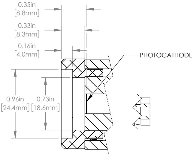
SECTION B-B SCALE 1.25 : 1
