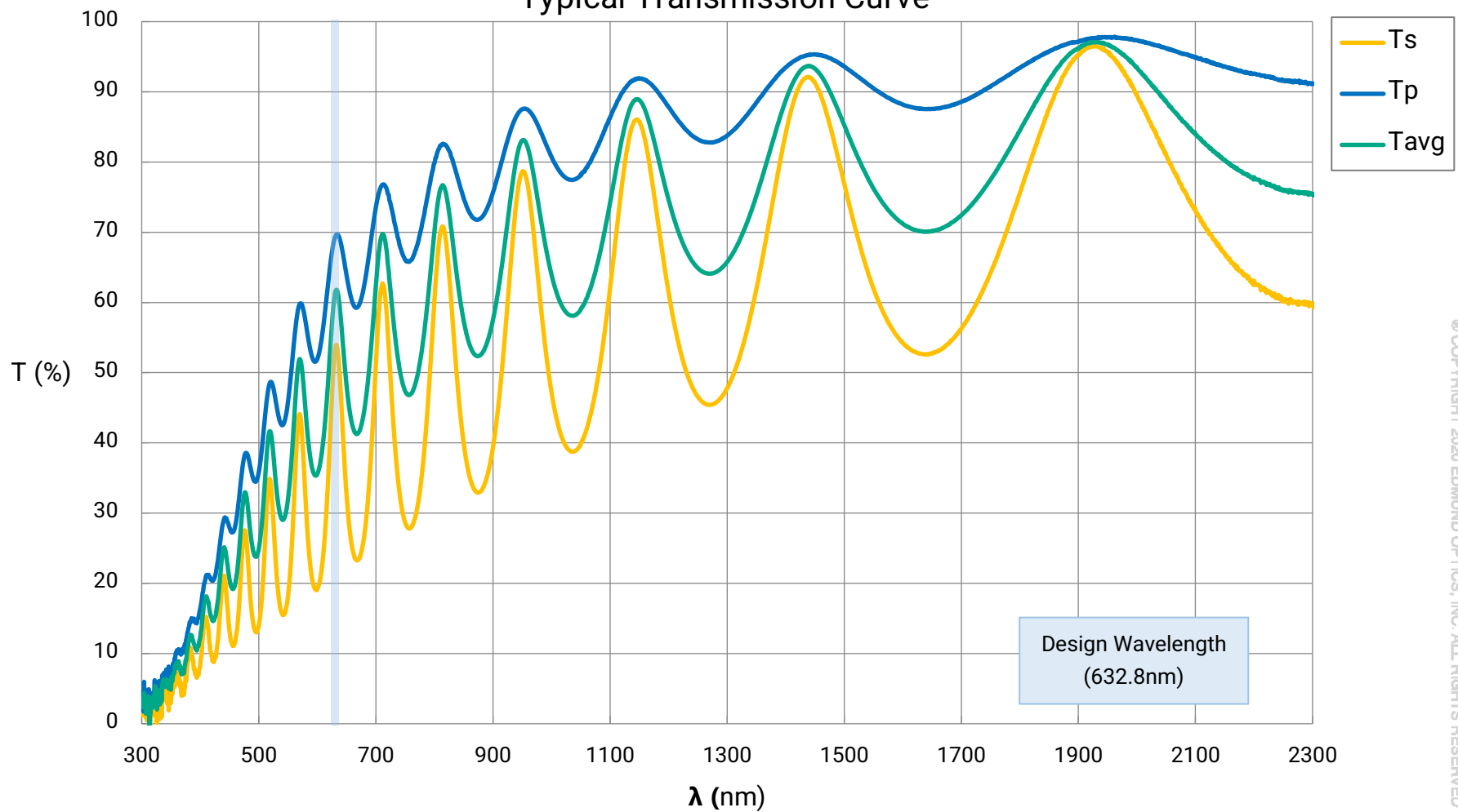
Dielectric Coated Pellicle Beamsplitter 50R/50T Splitting Ratio (632.8nm) Typical Transmission Curve
