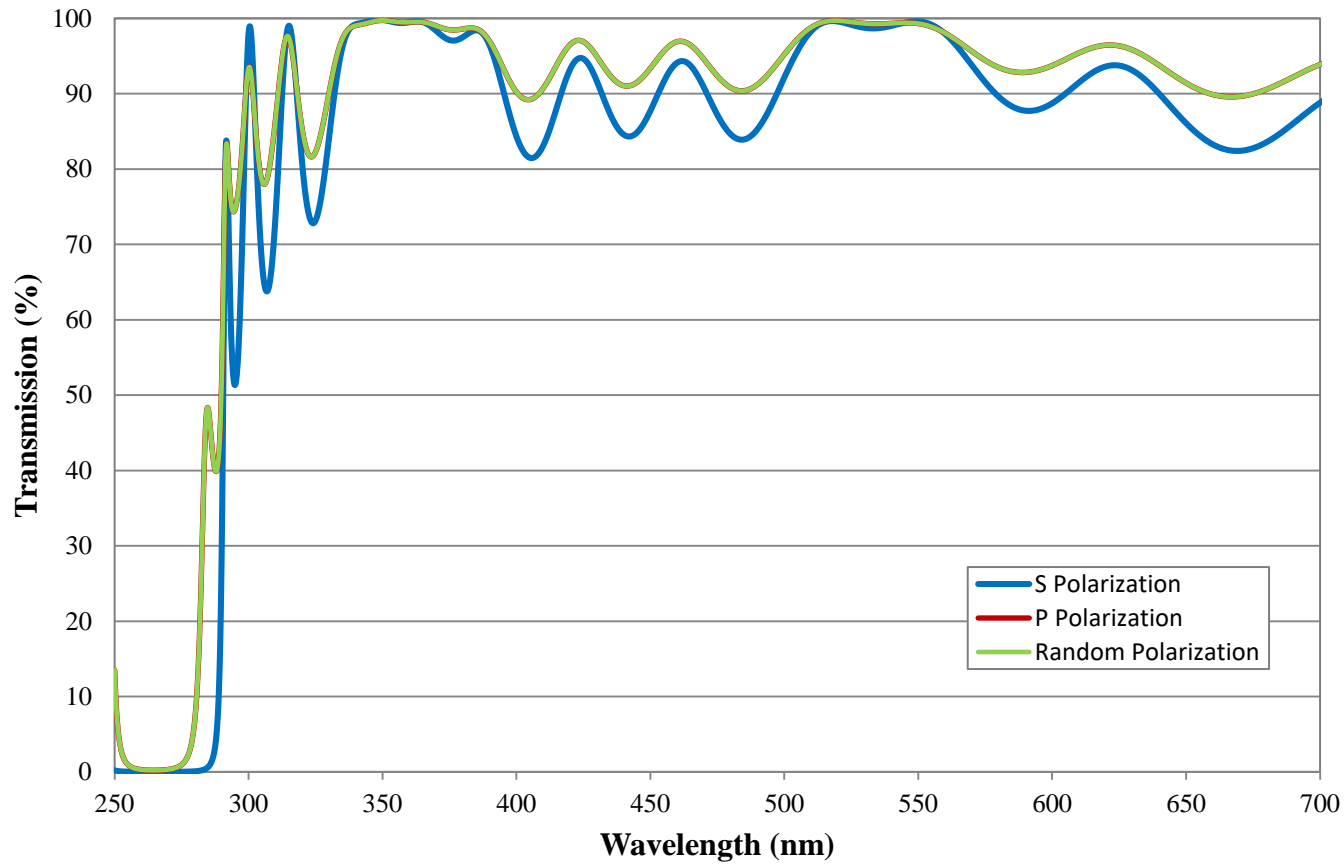
355nm T, 266nm R Harmonic Separator Typical Transmission FOR REFERENCE ONLY
