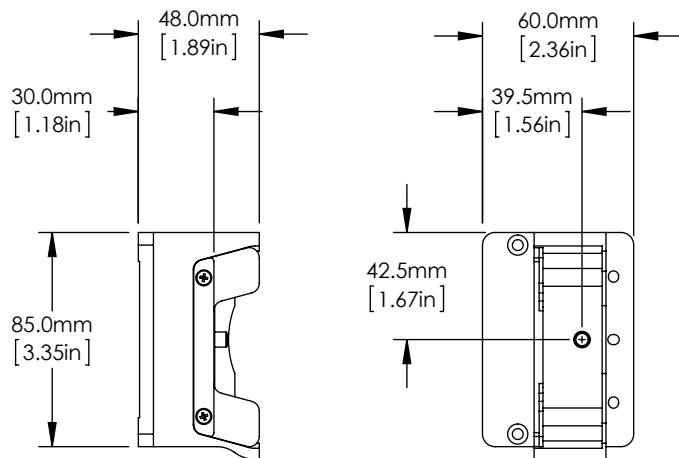
MOUNT FOR BC106 SERIES
