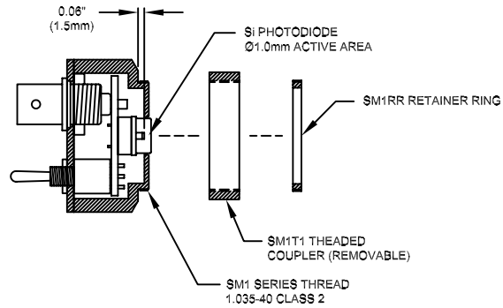
CROSS SECTION VIEW X-X
