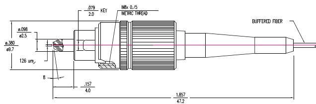
FC/APC Connector, Tight Fit Key, 900 \mu\text{m} Boot Style FC/APC Connector, Tight Fit Key, 90° Boot Style
