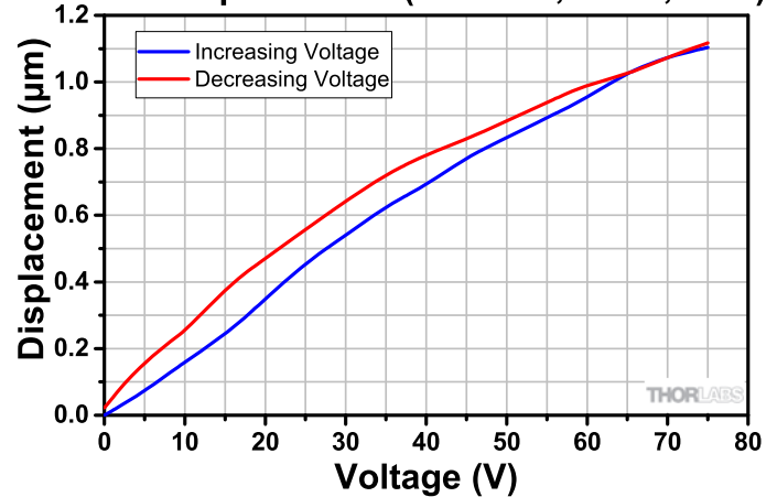
PA2AD Displacement (No Load, 25 °C, 75 V)
