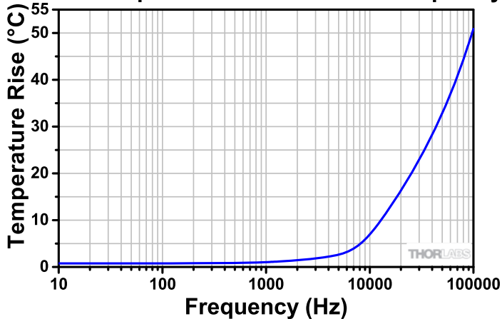
PA2AD Temperature Rise vs. Drive Frequency
