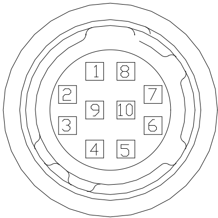
INTERFACE CONNECTOR
