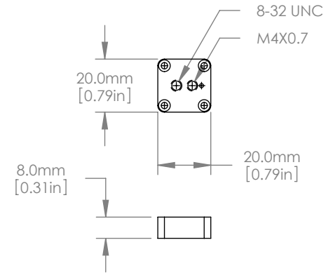
Adapter plate
