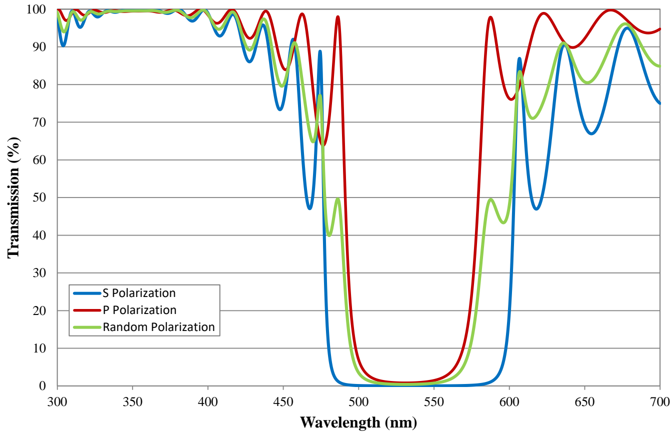
355nm T, 532nm R Harmonic Separator Typical Transmission FOR REFERENCE ONLY
