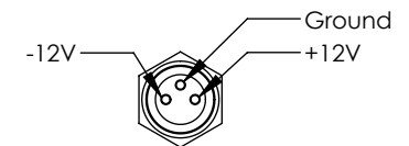
Electrical Connections
