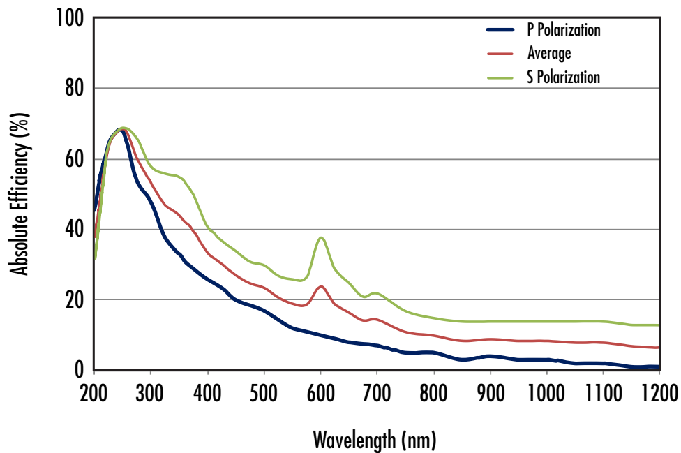
1200 Grooves/mm, VIS Holographic Grating Absolute Efficiency
