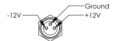
Electrical Connections
