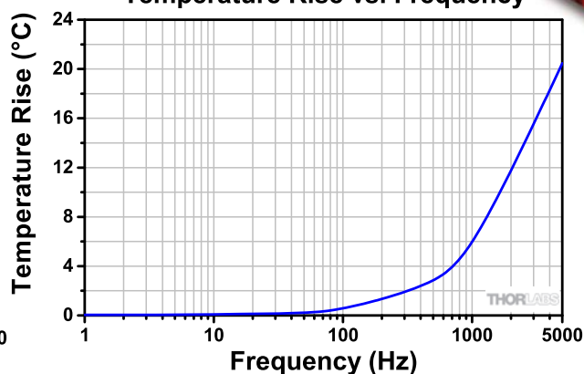
Temperature Rise vs. Frequency
