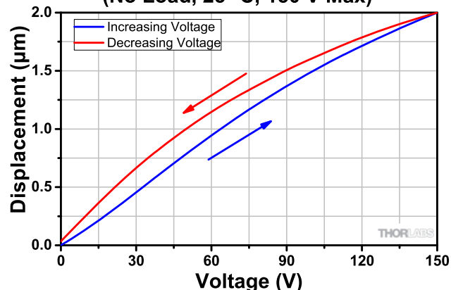
PA4GEH5(W) Displacement (No Load, 25 °C, 150 V Max)
