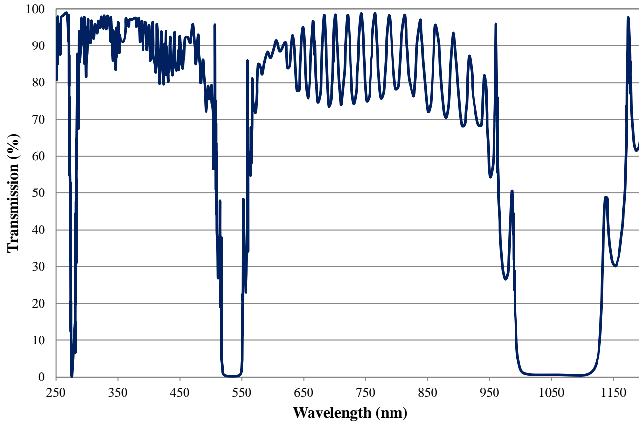
266nm T, 532 & 1064nm R Harmonic Separator Typical Transmission FOR REFERENCE ONLY
