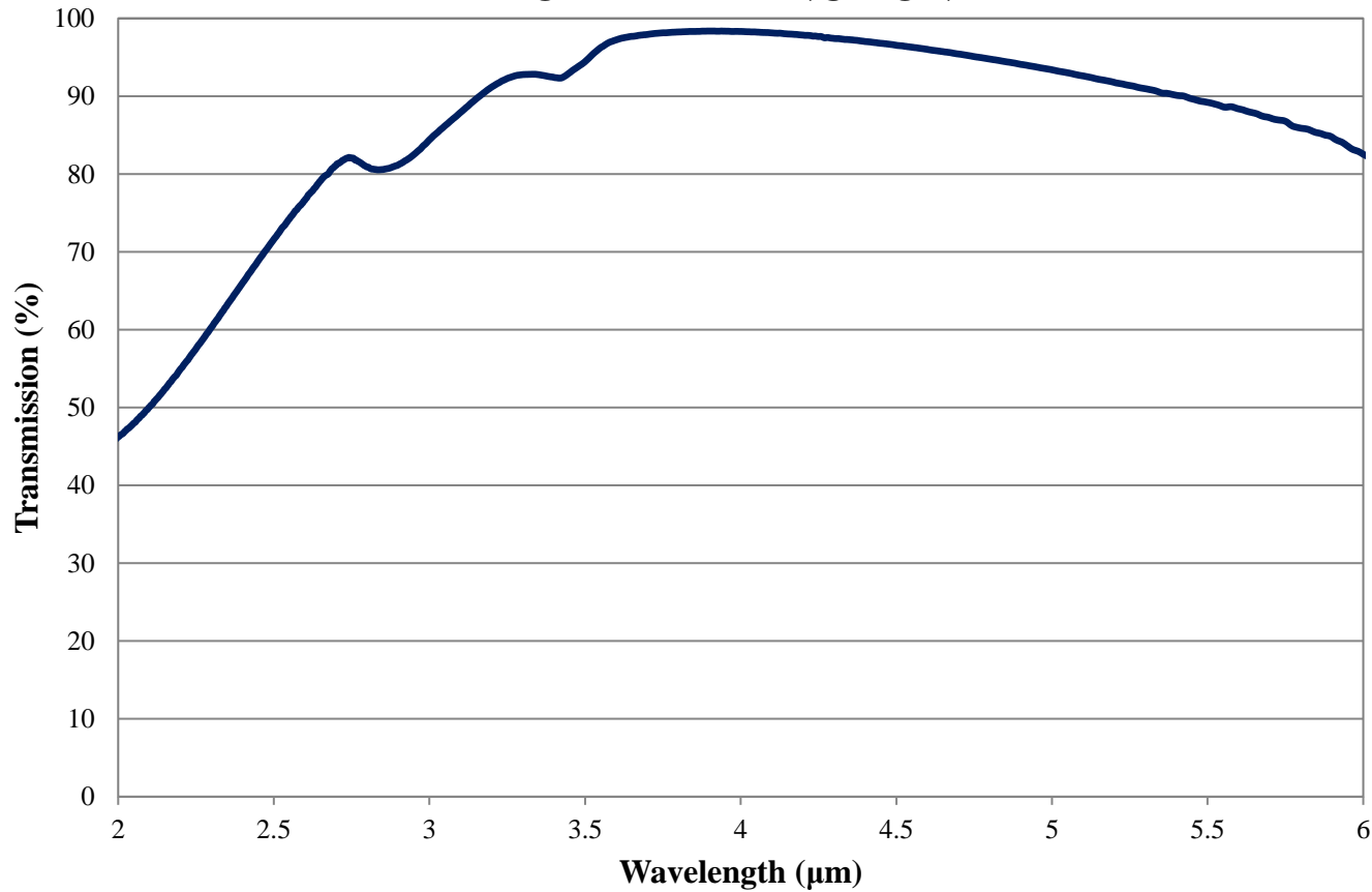
3-5 \mu m AR Coated & DLC Coated Si Window Typical Transmission FOR REFERENCE ONLY
