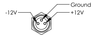
Electrical Connections
