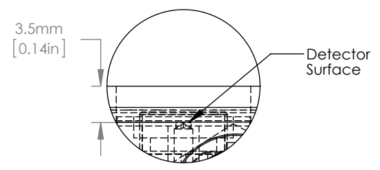
DETAIL A SCALE 2 : 1
